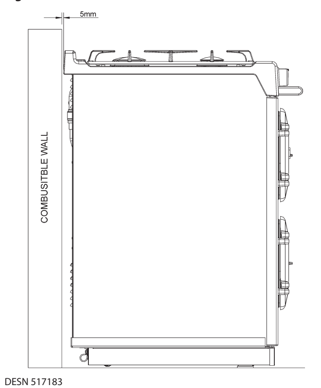
Fig. 12.4 COMBUSTIBLE WALL FITTING CLEARANCE
