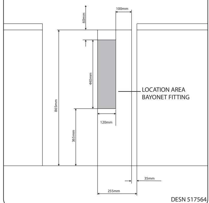
POSITION OF GAS BAYONET ON WALL Fig. 14.6 (locate in shaded areas)
