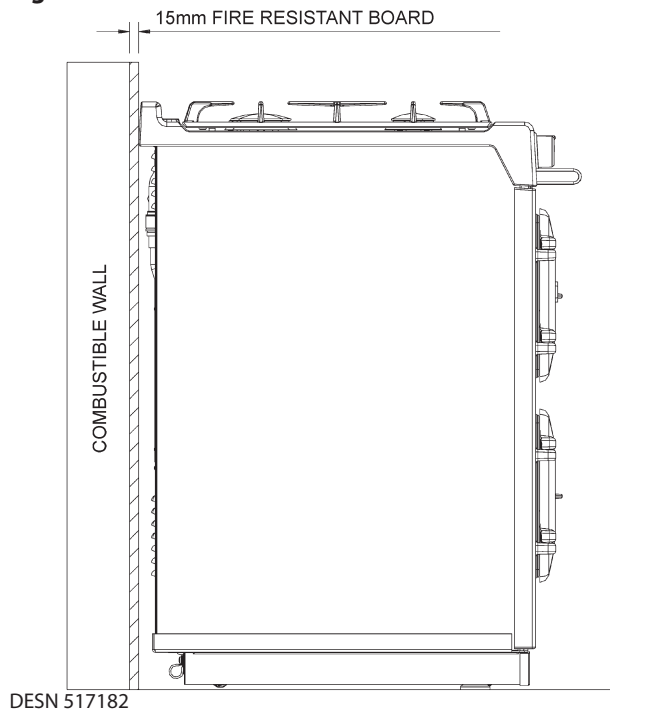
Fig. 12.3 COMBUSTIBLE WALL FITTING USING FIRE RESISTANT BOARD
